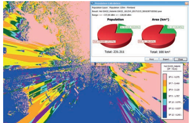
Coverage analysis assessing population and area covered
